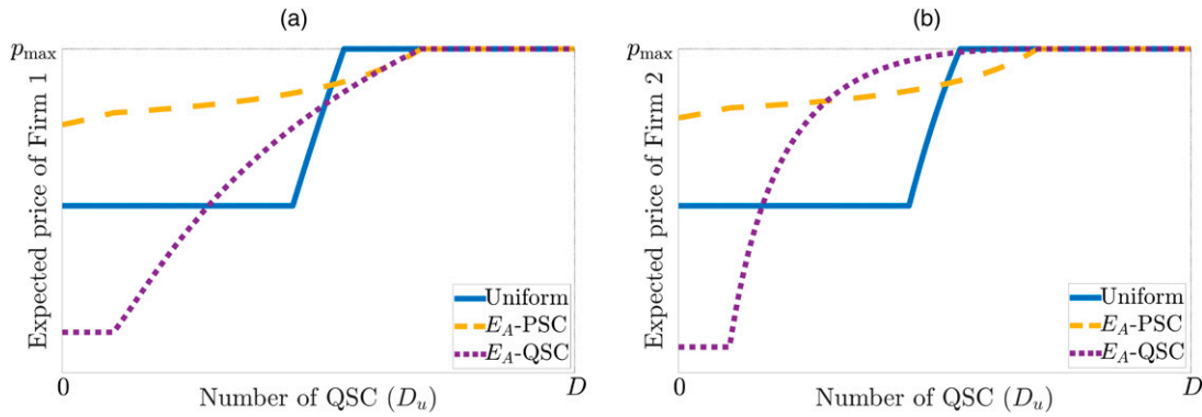
Figure 10. (Color online) Expected Prices When \left(2 - \frac{\Delta}{p_{\max}}\right)I \leq D < \frac{4p_{\max}-3\Delta}{2p_{\max}-\Delta}I ( D = 20 , p_{\max} = 20 , I = 11 , \Delta = 5 )
