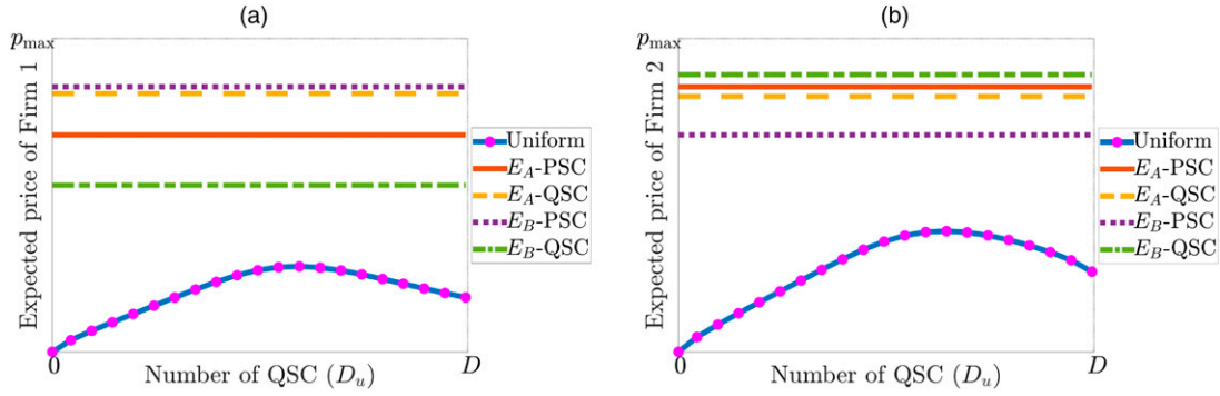
Figure 6. (Color online) Expected Prices Comparisons Under Low Demand (Parameters: D = 20 , p_{\max} = 20 , \Delta = 5 )
